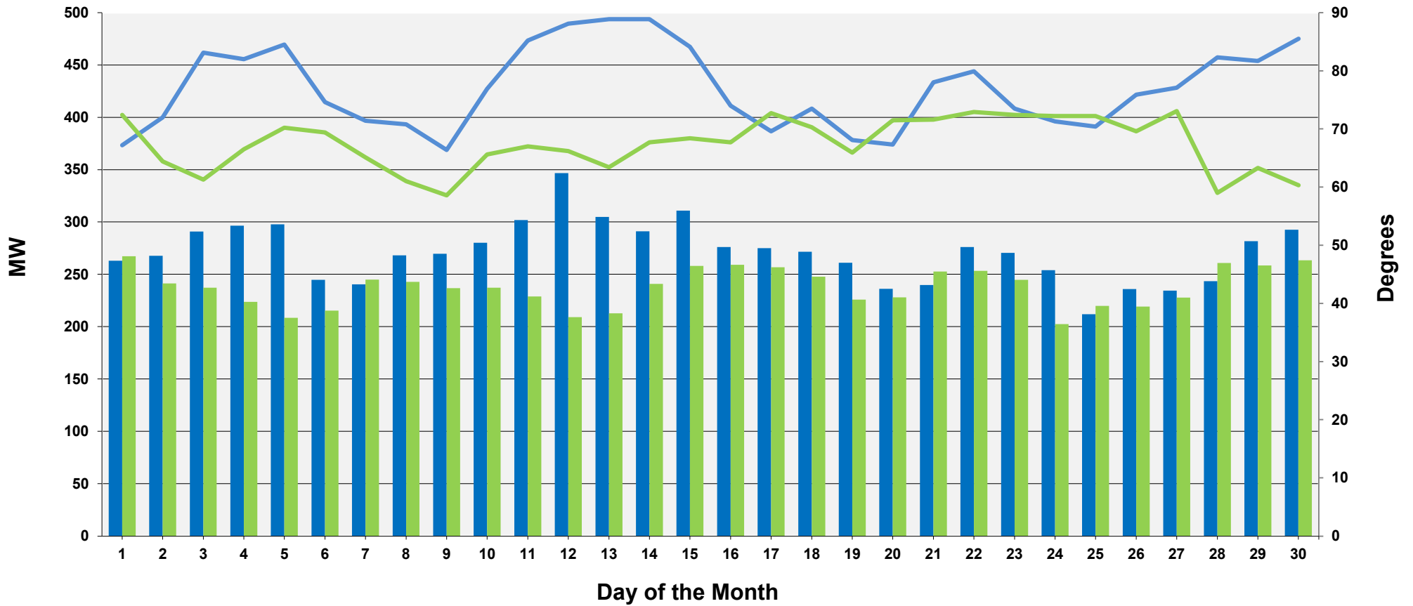
Chart 4 Daily Peak Load and Temperature Comparisons November
