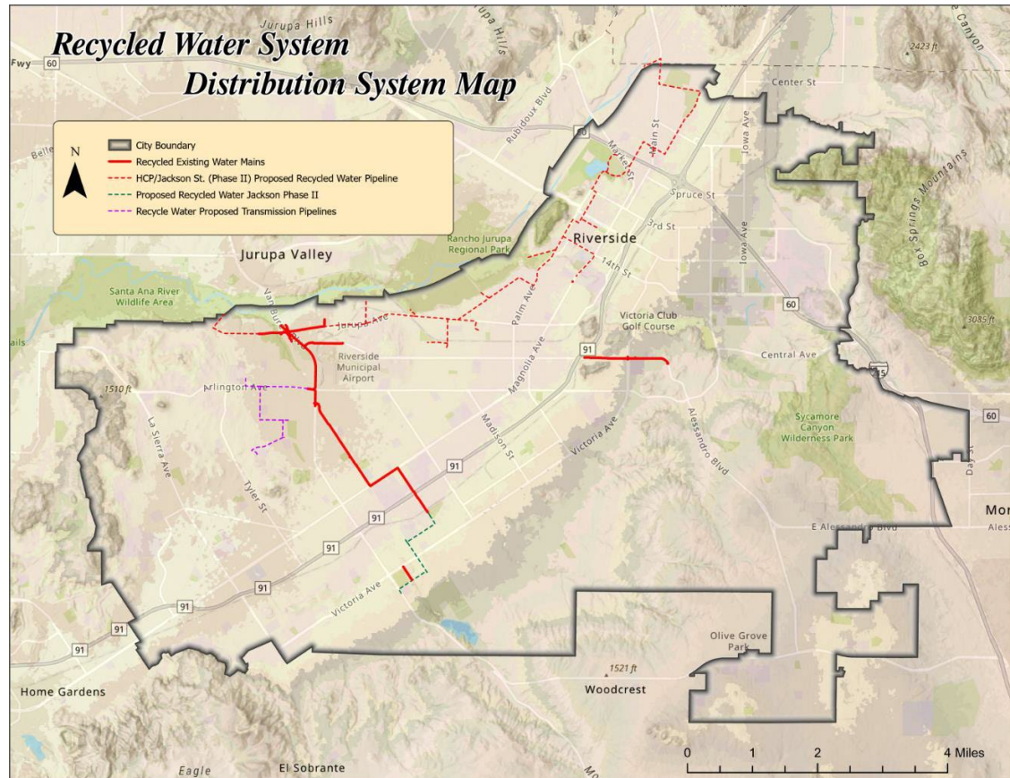
Figure 6-1 – Recycled Water Distribution System (Existing and Proposed)
