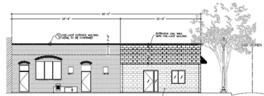
PROPOSED SOUTH ELEVATION Scale: 1/8" = 1'-0"
