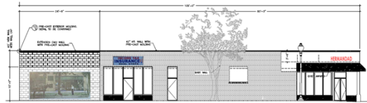
PROPOSED VAN BUREN'S (EAST) ELEVATION Scale: 1/8" = 1'-0"
