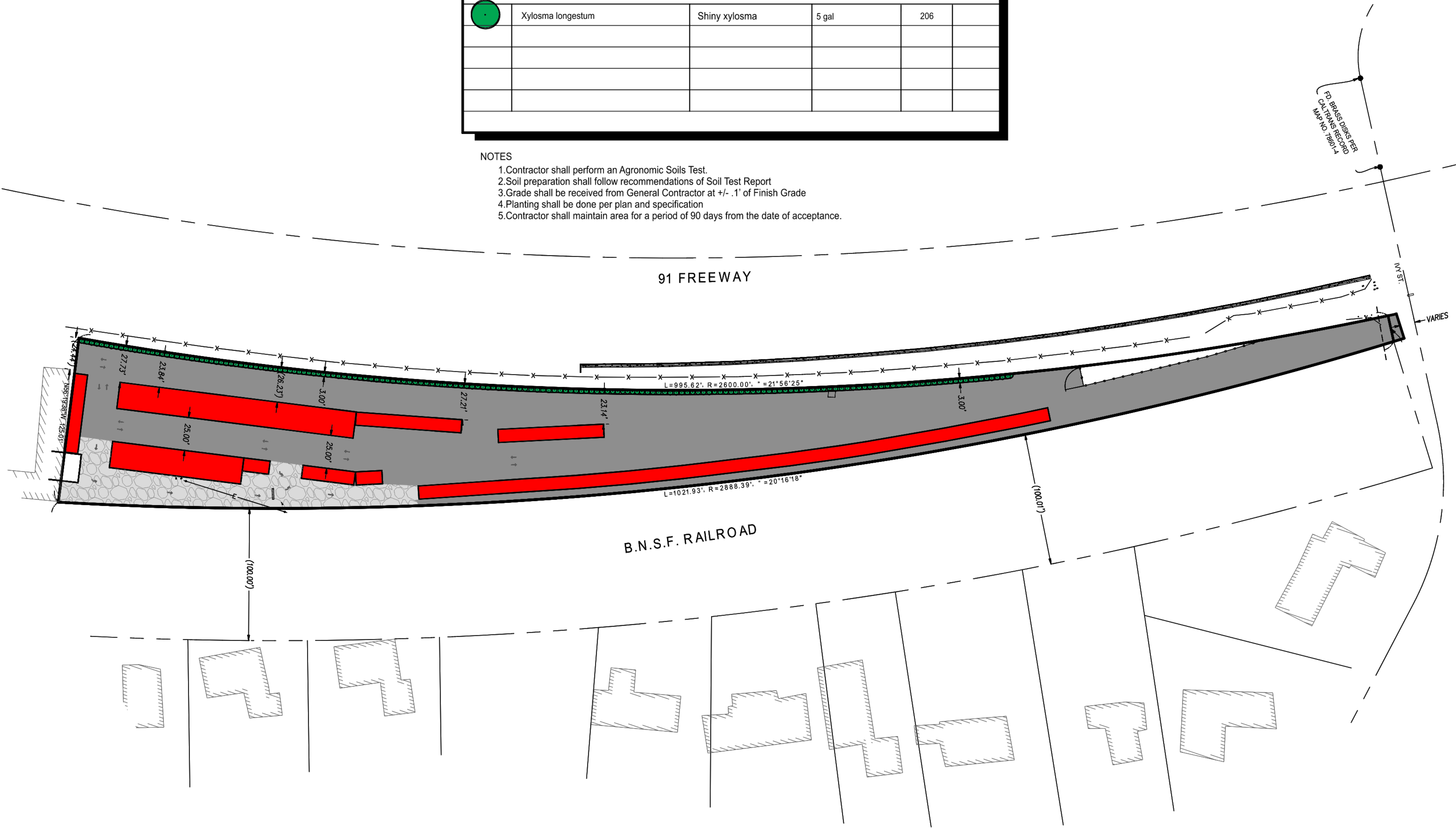
LANDSCAPE PLAN
