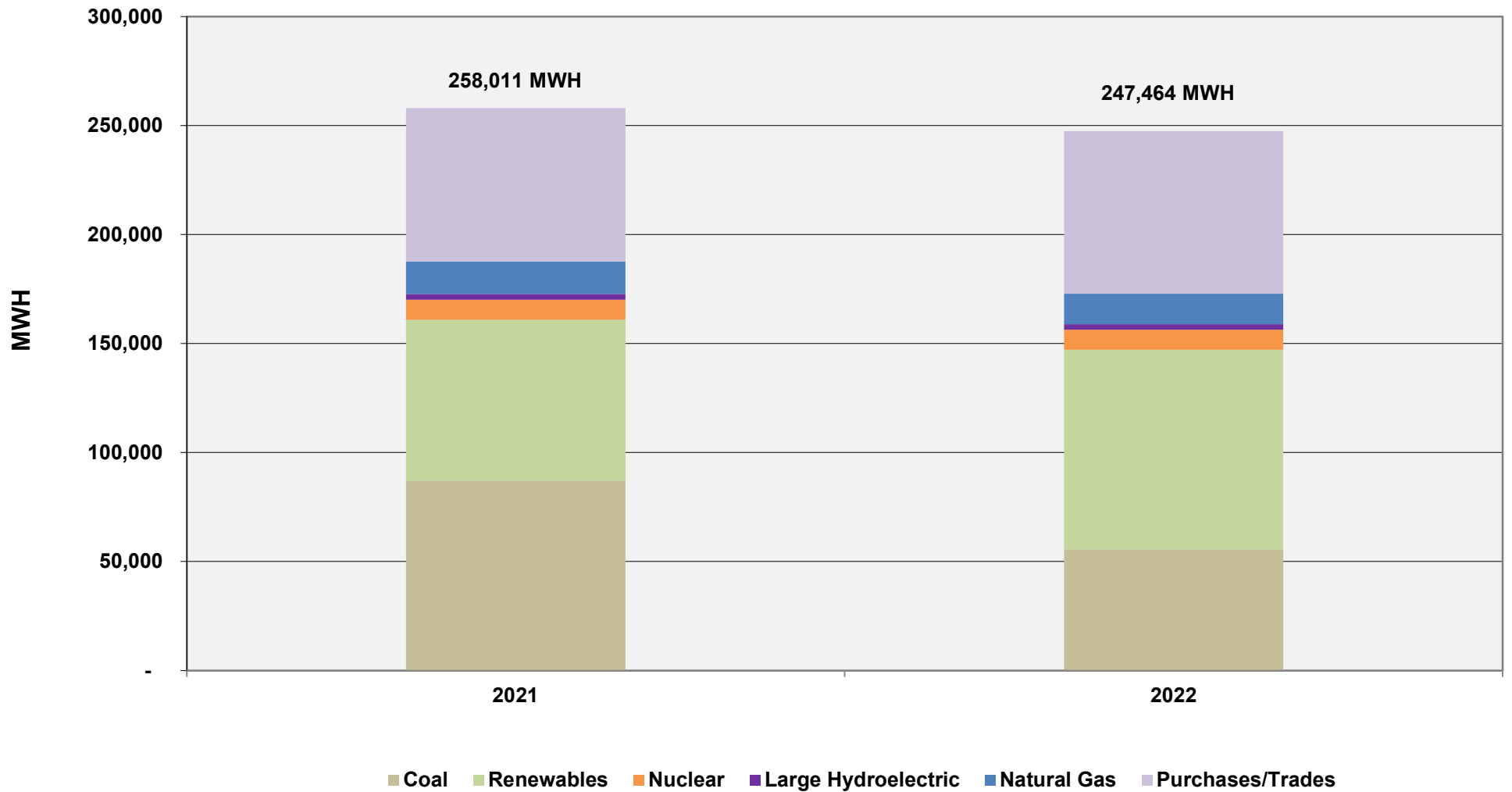
Chart 1 Total Energy Requirements/Resource Mix - July
