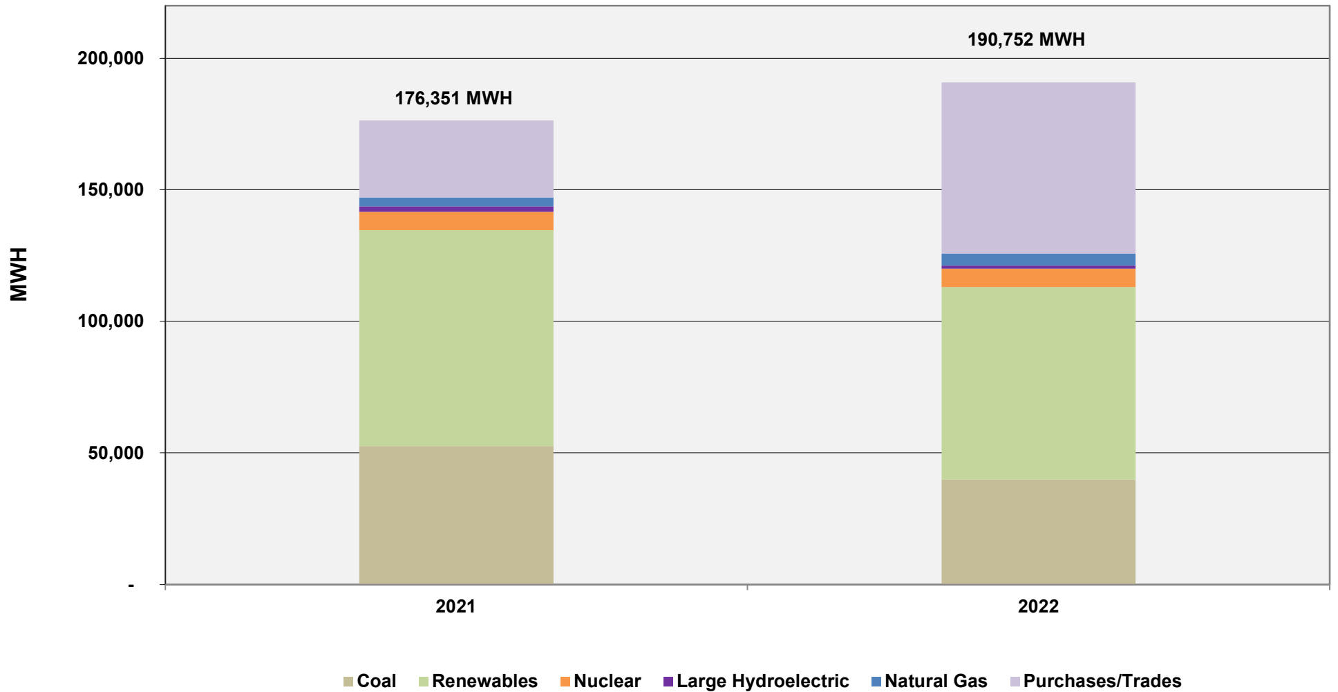
Chart 1 Total Energy Requirements/Resource Mix - October
