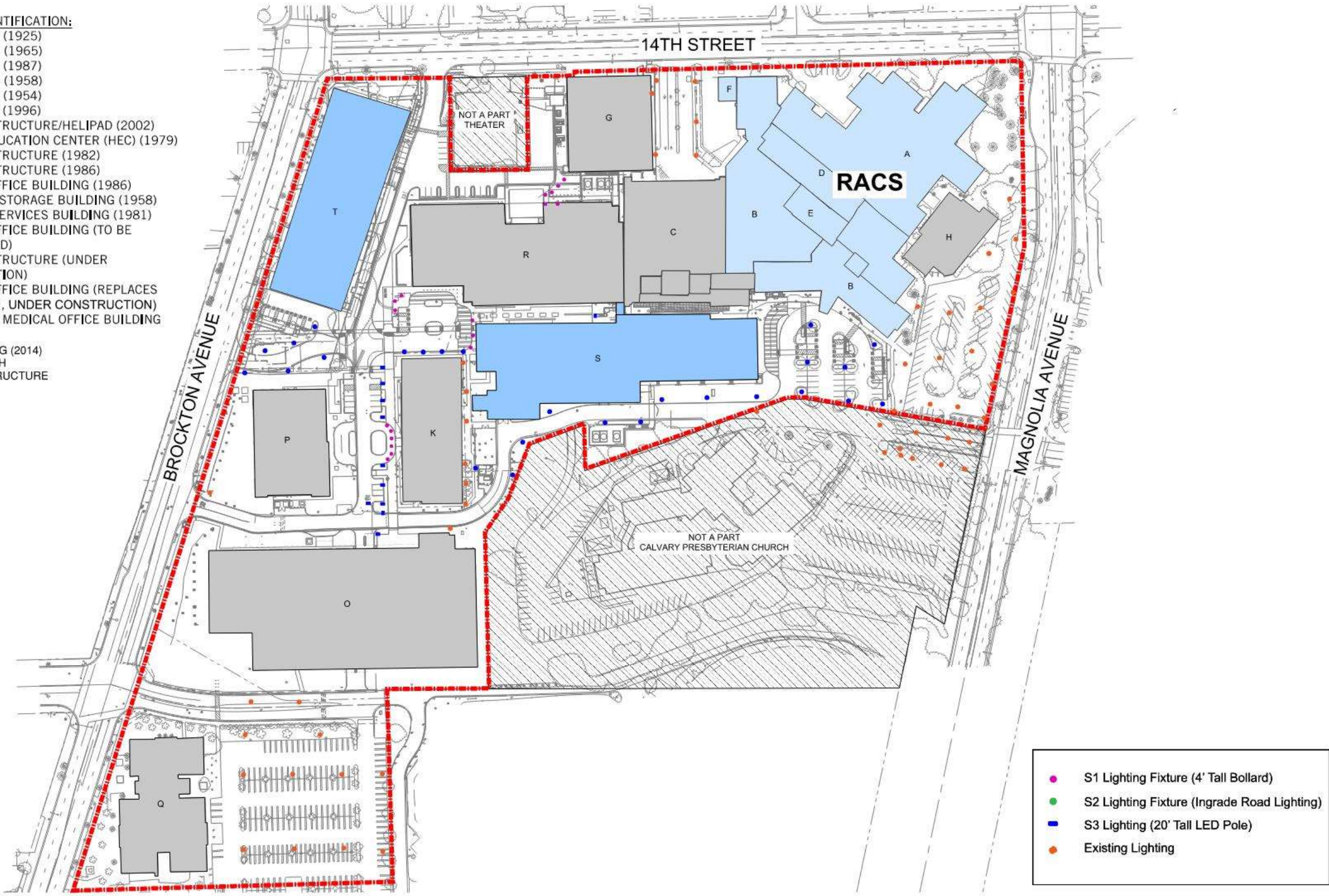
FIGURE 8-6 Lighting Plan
