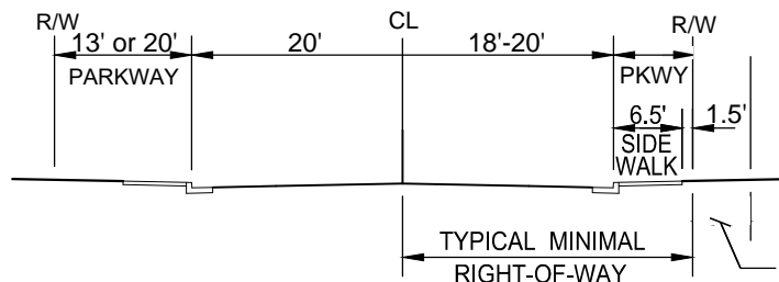
MODIFIED ROADWAY CROSS-SECTION
