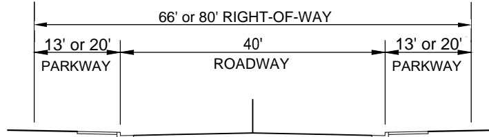
STANDARD ROADWAY CROSS-SECTION
