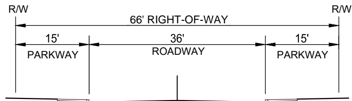
STANDARD ROADWAY CROSS-SECTION
