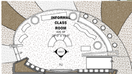
1 Floor Plan Scale: 0' to 10'
