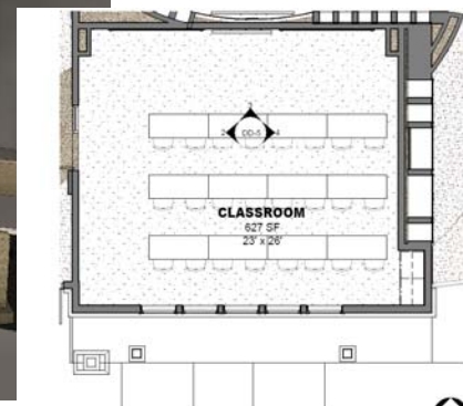
1 Floor Plan Scale: 0' to 10'
