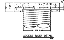
ACCESS RISER DETAIL
