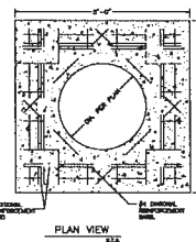
PLAN VIEW
