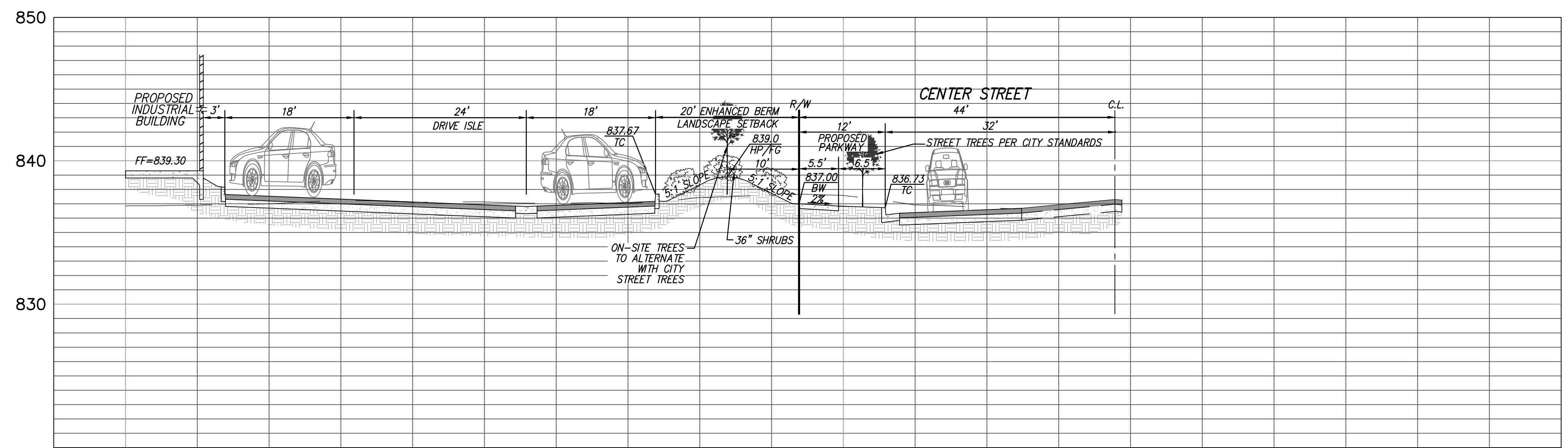
PROPOSED CENTER STREET TYPICAL SECTION SCALE: HORIZONTAL : 1"=10' VERTICAL : 1"=5'
