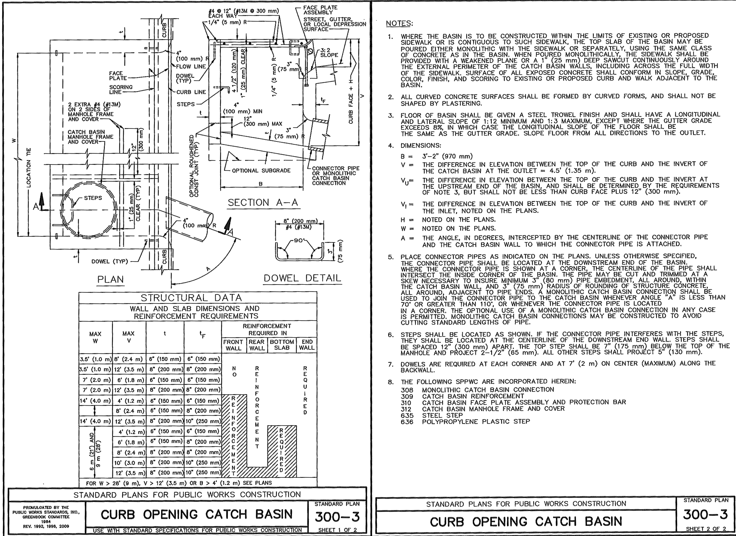
CURB OPENING CATCH BASIN N.T.S.
