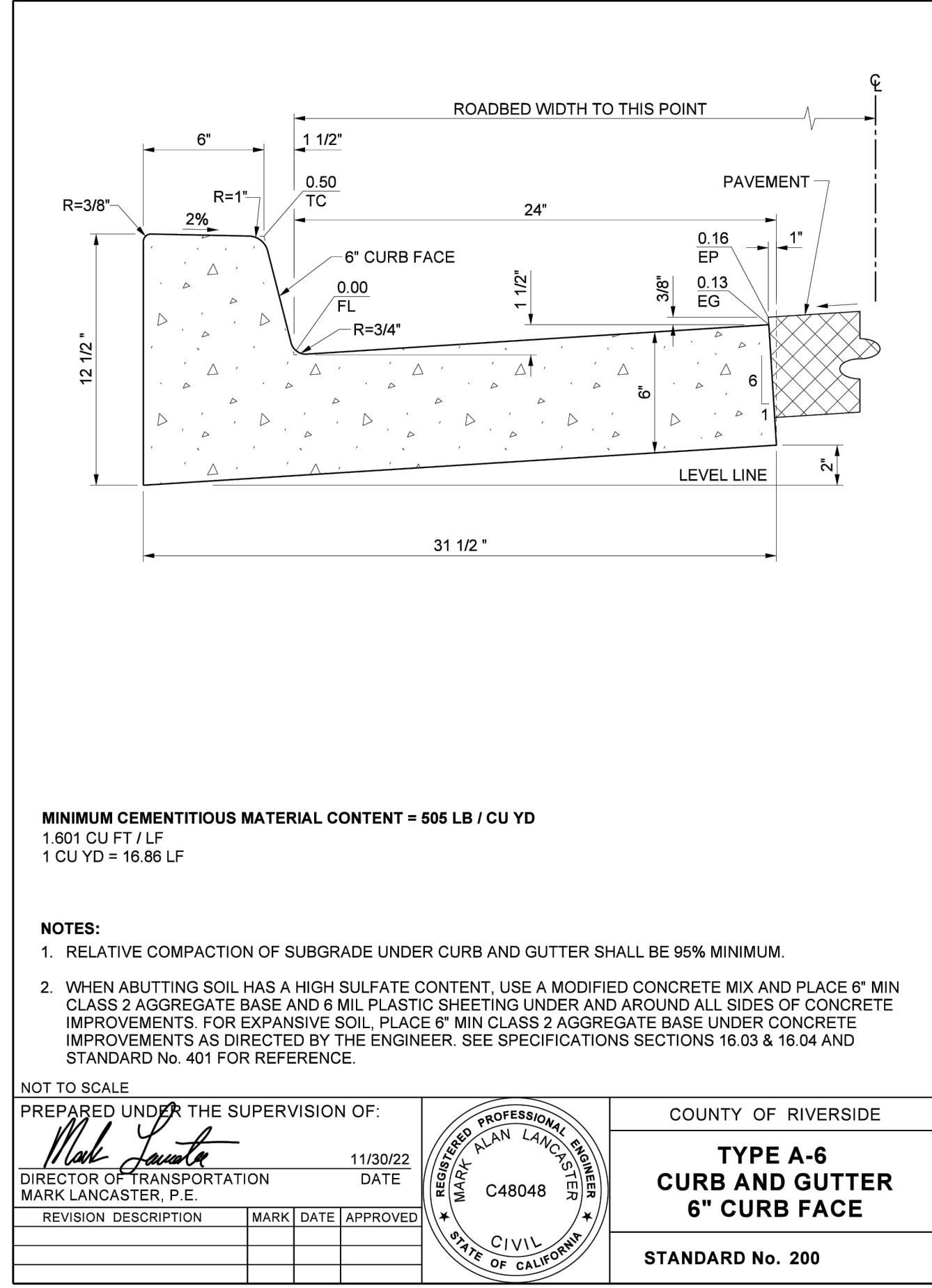
CITY OF RIVERSIDE 6" CURB AND GUTTER DETAIL N.T.S.
