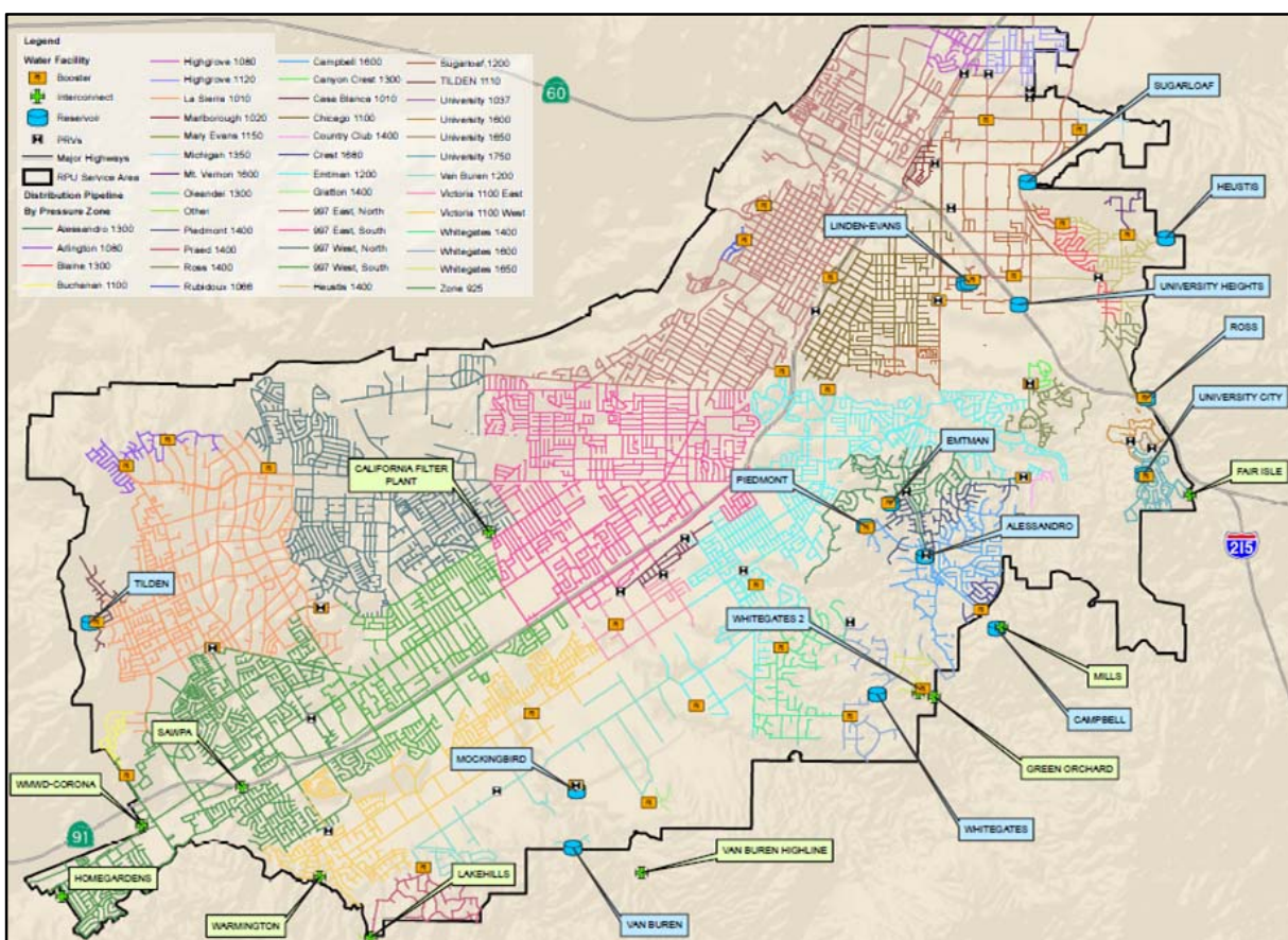
FIGURE 2-4 DISTRIBUTION SYSTEM
