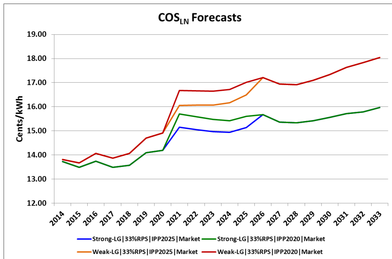
Figure 10.4.1. Projected annual COS_{LN} estimates for two load growth assumptions and IPP contract end-dates: (strong versus weak load growth & December 31, 2020 versus December 31, 2025), assuming a 33% RPS mandate.
