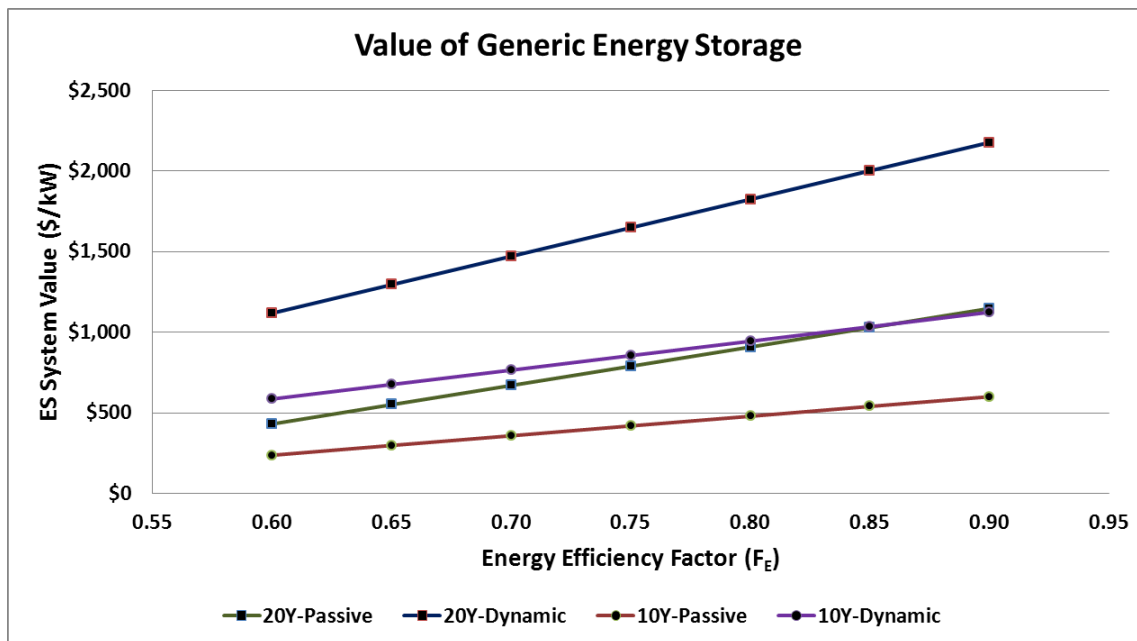
Figure 14.1.10. Forecasted NPV relationships for generic passive and dynamic energy storage systems, for an assumed FAS ratio of 0.5 and an annual discount rate of 3%.
