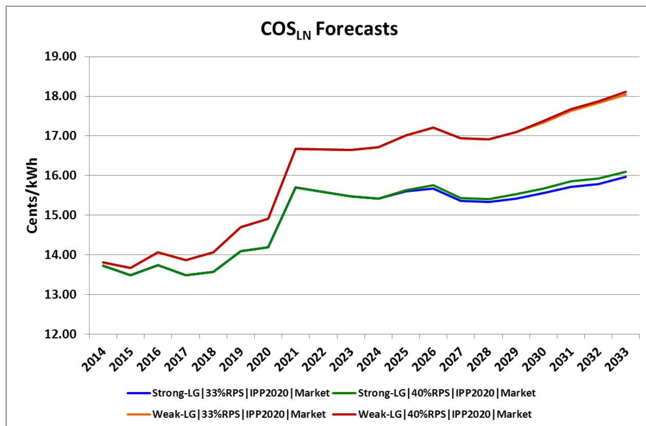
Figure 10.3.3. Projected annual COS LN estimates for two load growth assumptions and RPS mandates: (strong versus weak load growth & 33% versus 40% RPS mandates), assuming a 2020 IPP contract termination date.
