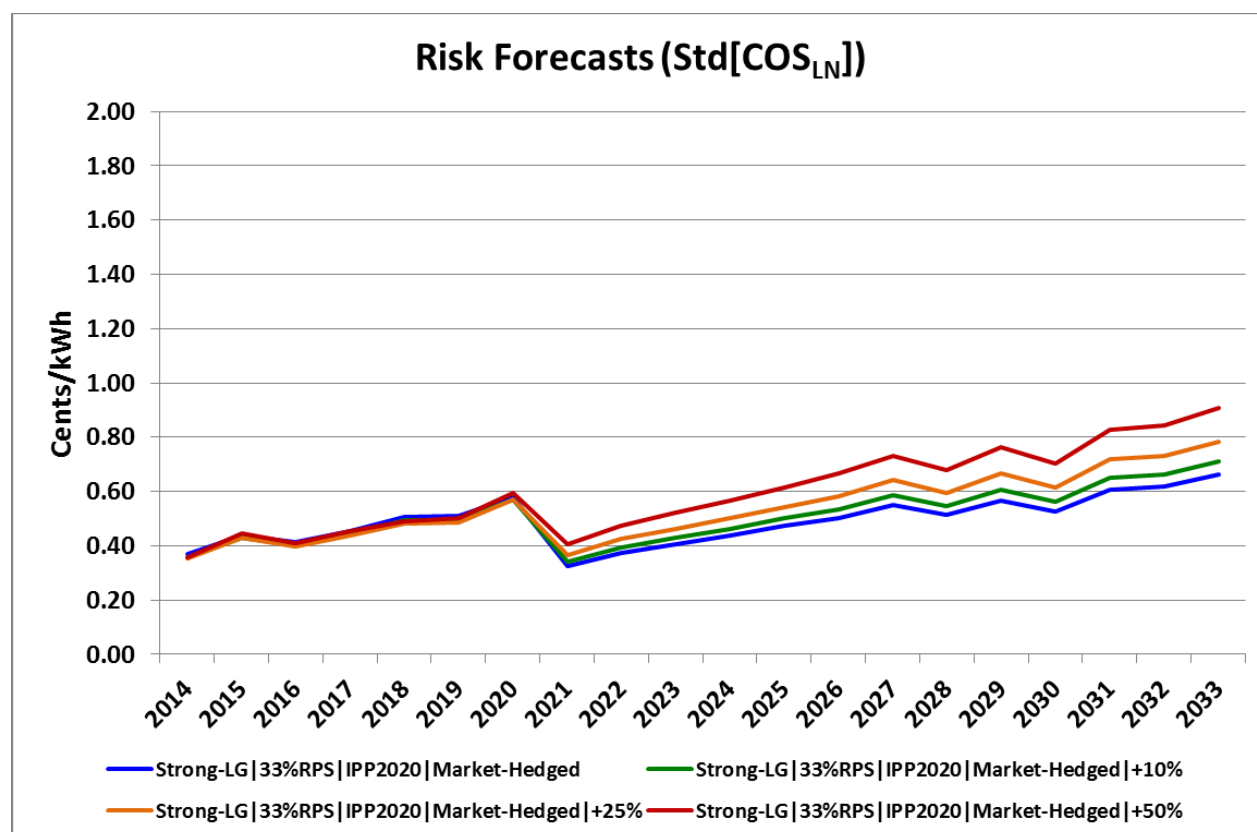
Figure 10.6.4. Corresponding annual COS LN risk estimates (Std[COS LN ]) for the baseline and three market price shock scenarios shown in Figure 10.6.3, assuming strong load growth, a 33% RPS mandate, a 2020 IPP contract termination date, and 150 MW of forward hedged energy contracts as an IPP replacement option.
