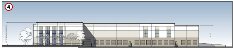
West Elevation
