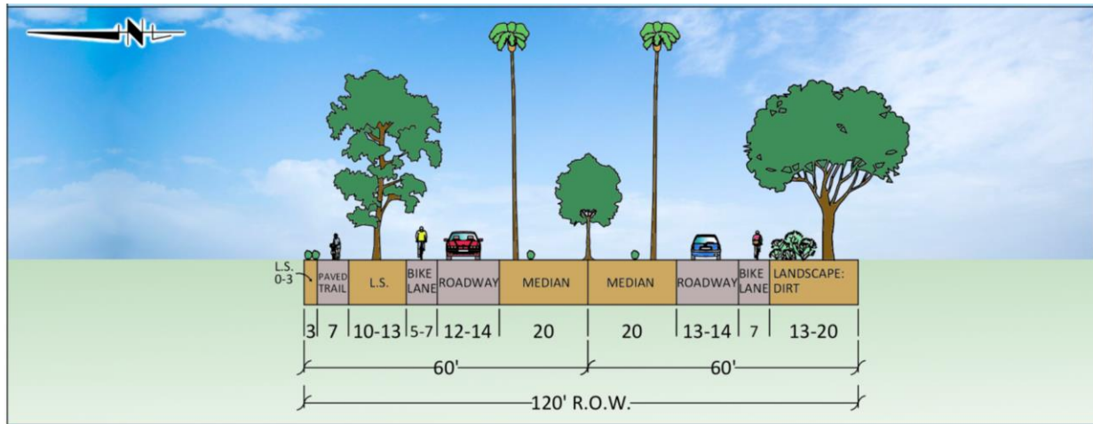
Figure 1 - Cross Section: Existing Typical Undeveloped R.O.W. Condition
