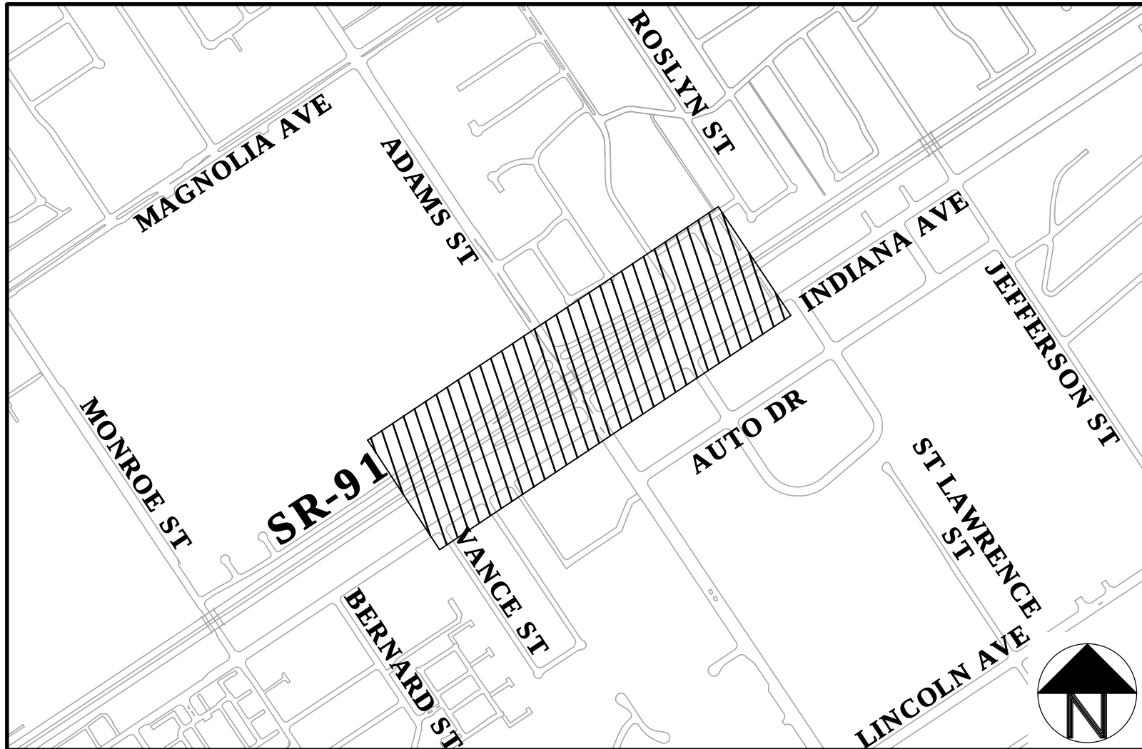
LOCATION MAP ADAMS STREET/SR-91 INTERCHANGE
