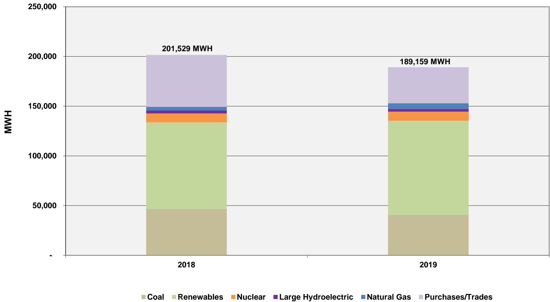
Chart 1 Total Energy Requirements/Resource Mix - June
