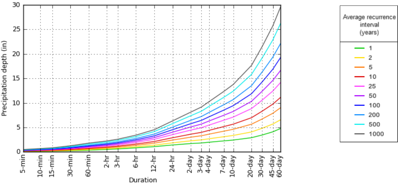
PDS-based depth-duration-frequency (DDF) curves Latitude: 33.9210°, Longitude: -117.3051°
