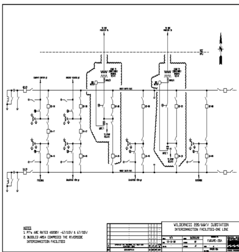
Exhibit E Riverside Wilderness Substation One-Line Diagram
