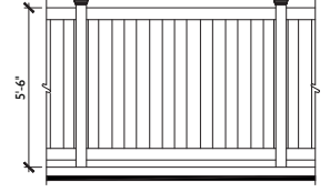
B VINYL PRIVACY FENCE 5'-6" HIGH
