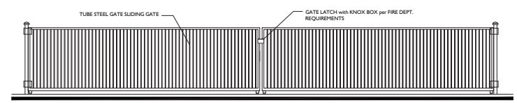
E DECORATIVE EVA GATE (MANUAL) 3'-6" HIGH
