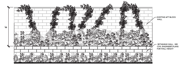
F RETAINING CONDITION AT PERIMETER +/- 2'-8" HIGH
