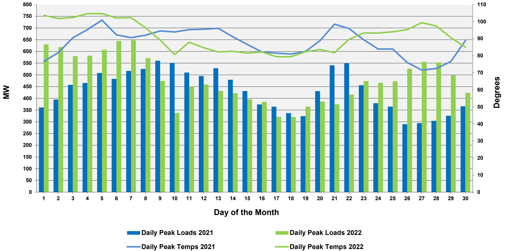
Chart 4 Daily Peak Load and Temperature Comparisons September
