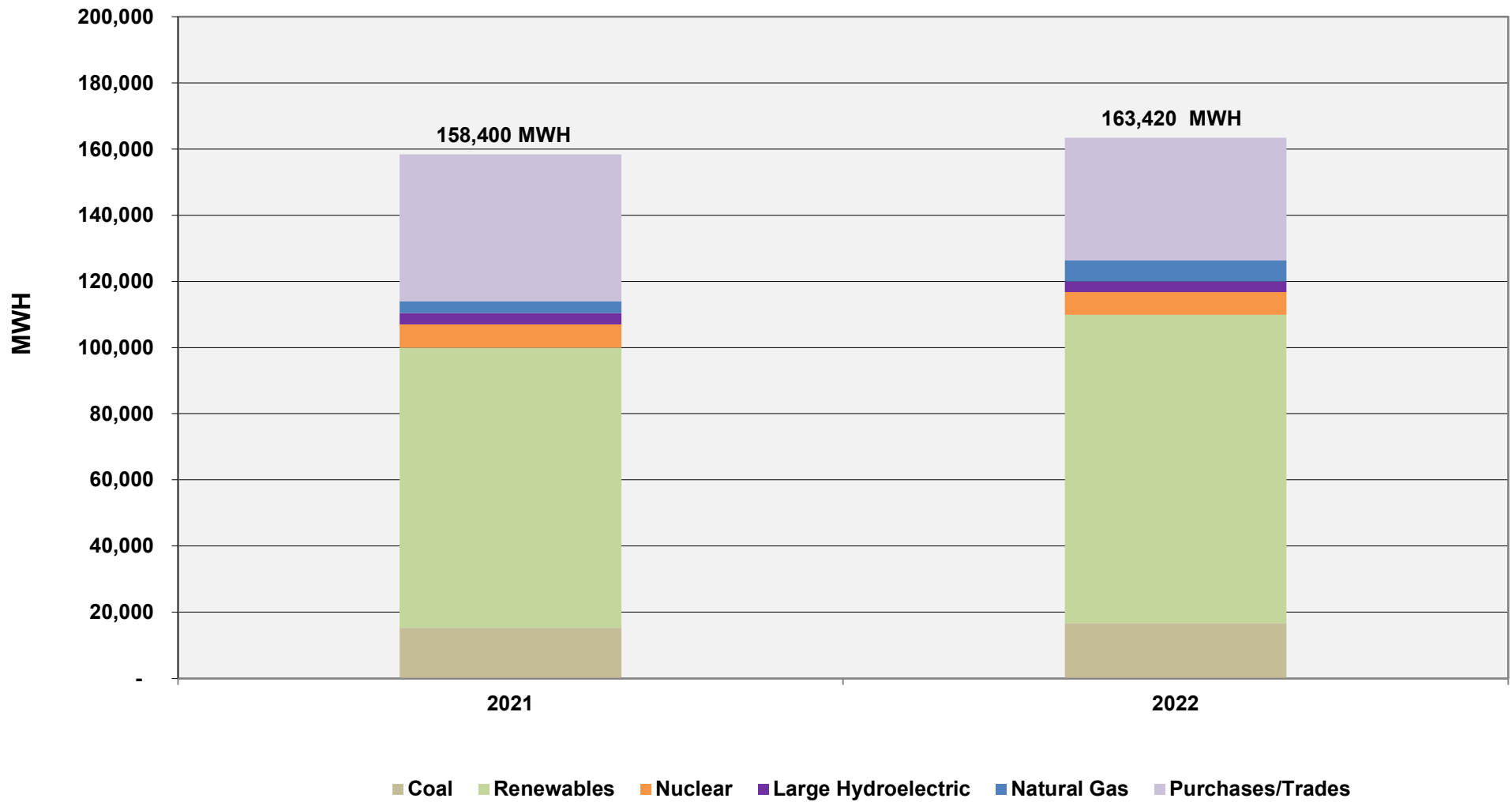
Chart 1 Total Energy Requirements/Resource Mix - April
