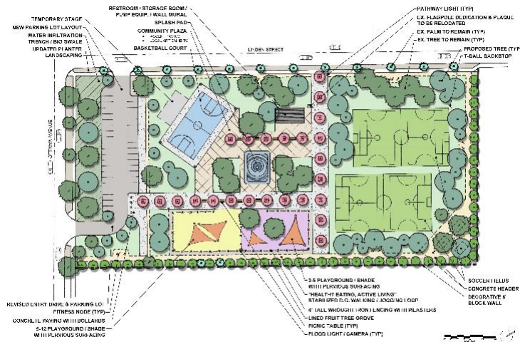
PATTERSON PARK CONCEPTUAL MASTER PLAN
