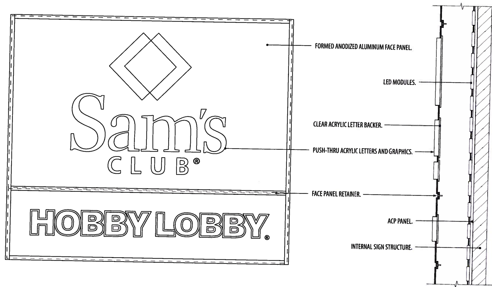
TYPICAL REMOVABLE SIGN FACE SCALE: 1/4"=1'-0"
