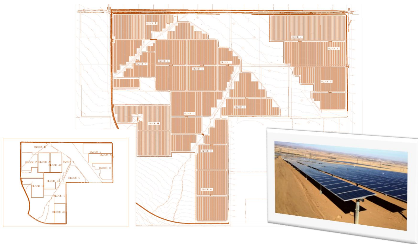
Figure 3 - Antelope DSR I Site Layout & Photo
