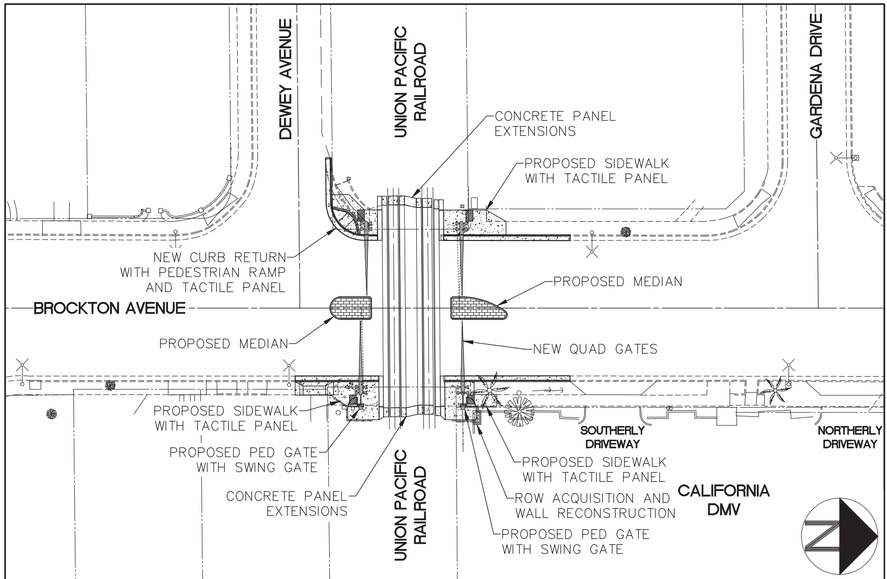
QUIET ZONE IMPROVEMENTS FOR BROCKTON AVENUE AT UNION PACIFIC RAILROAD CROSSING (ALTERNATIVE 1)
