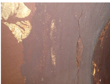
Circumferential pipe crack
