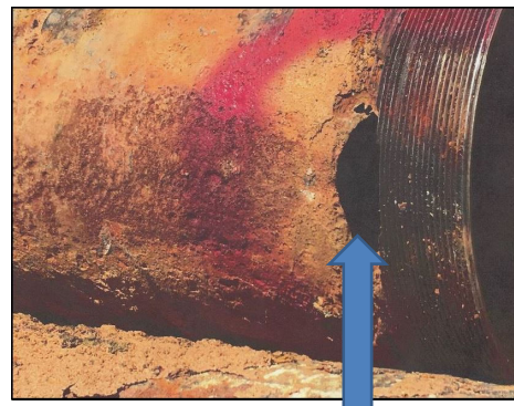
Large hole in section of column pipe
