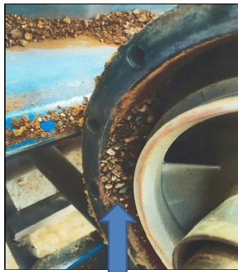
Sand and gravel in the pump assembly
