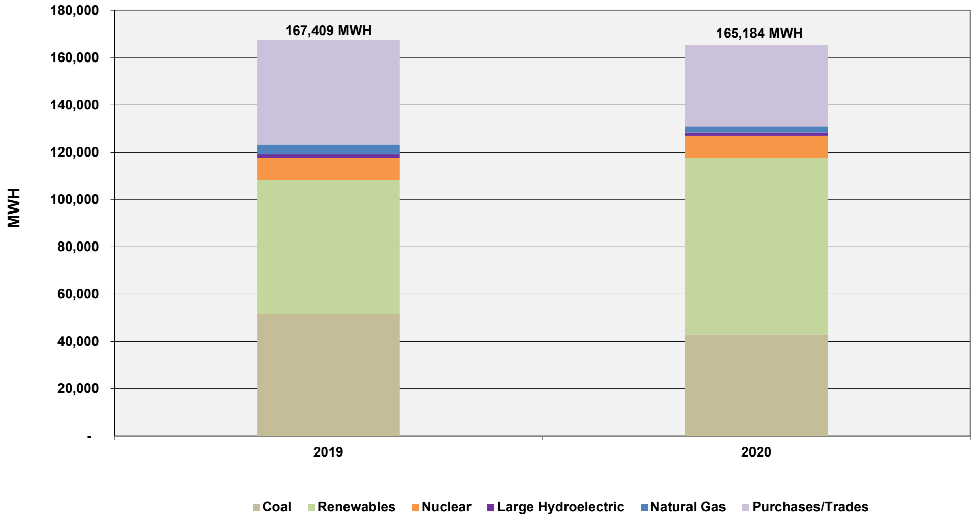
Chart 1 Total Energy Requirements/Resource Mix - January
