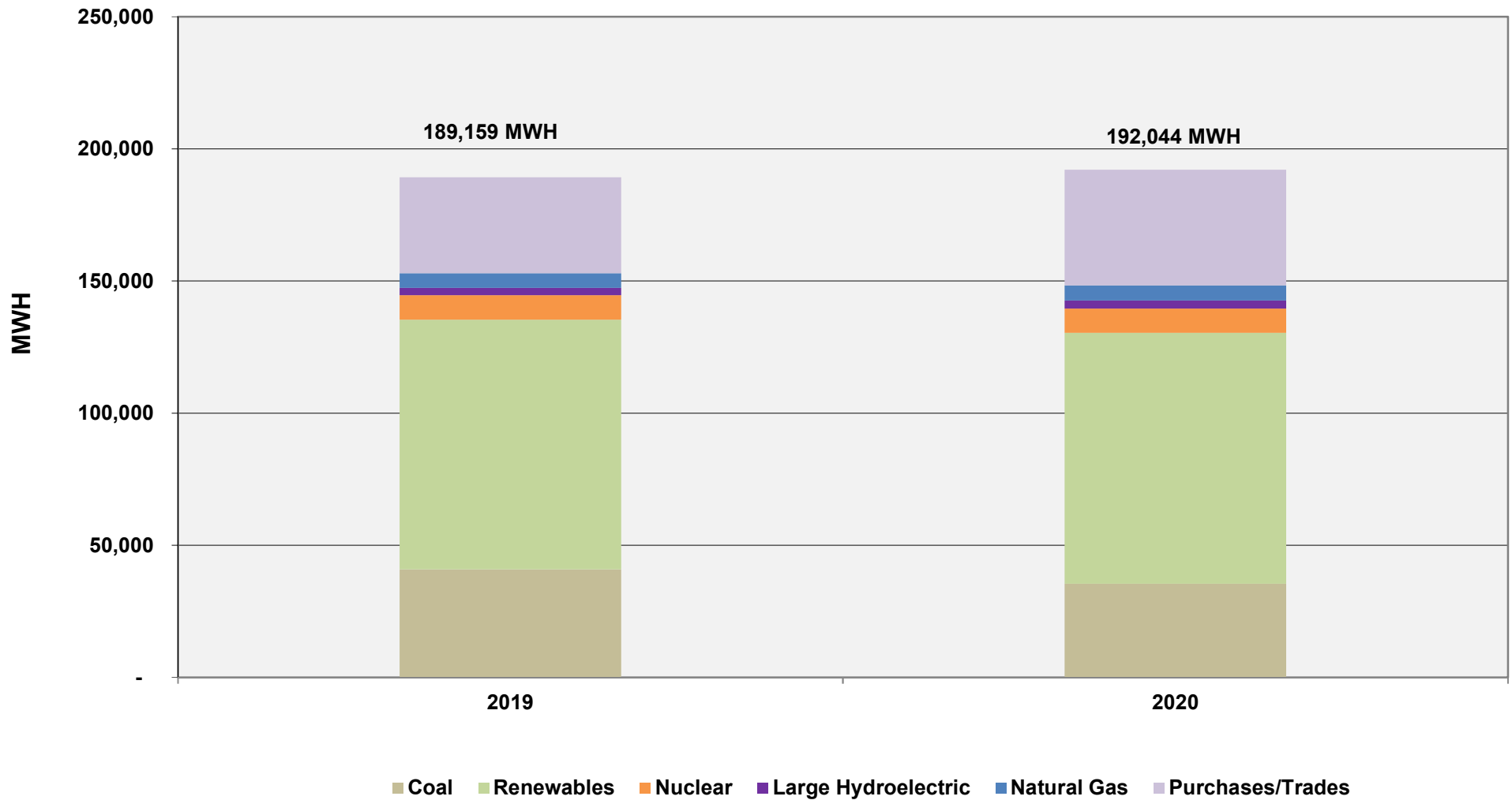
Chart 1 Total Energy Requirements/Resource Mix - June
