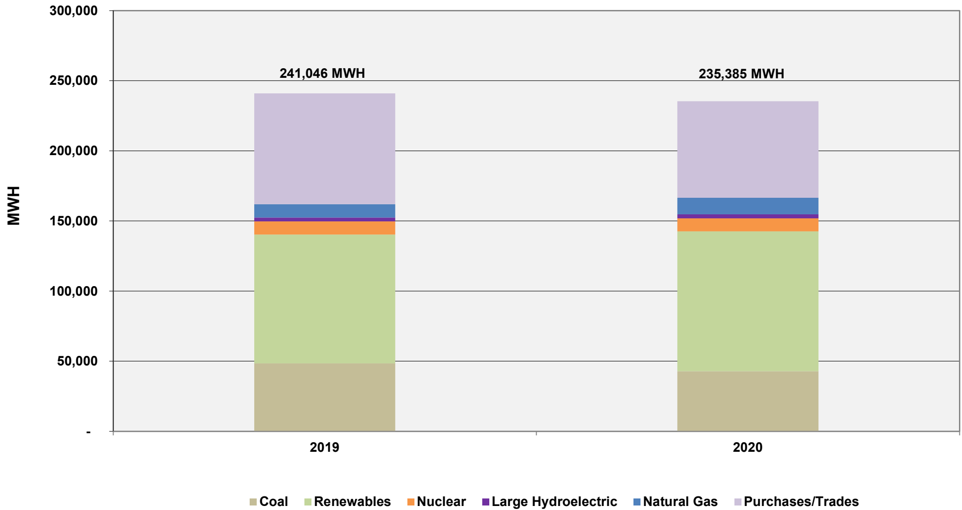
Chart 1 Total Energy Requirements/Resource Mix - JULY
