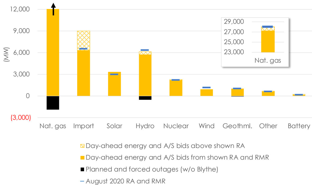
Figure B.9: August 14 Net Load Peak (6:51 pm) – Day-Ahead Bids vs. August 2020 Shown RA and RMR
