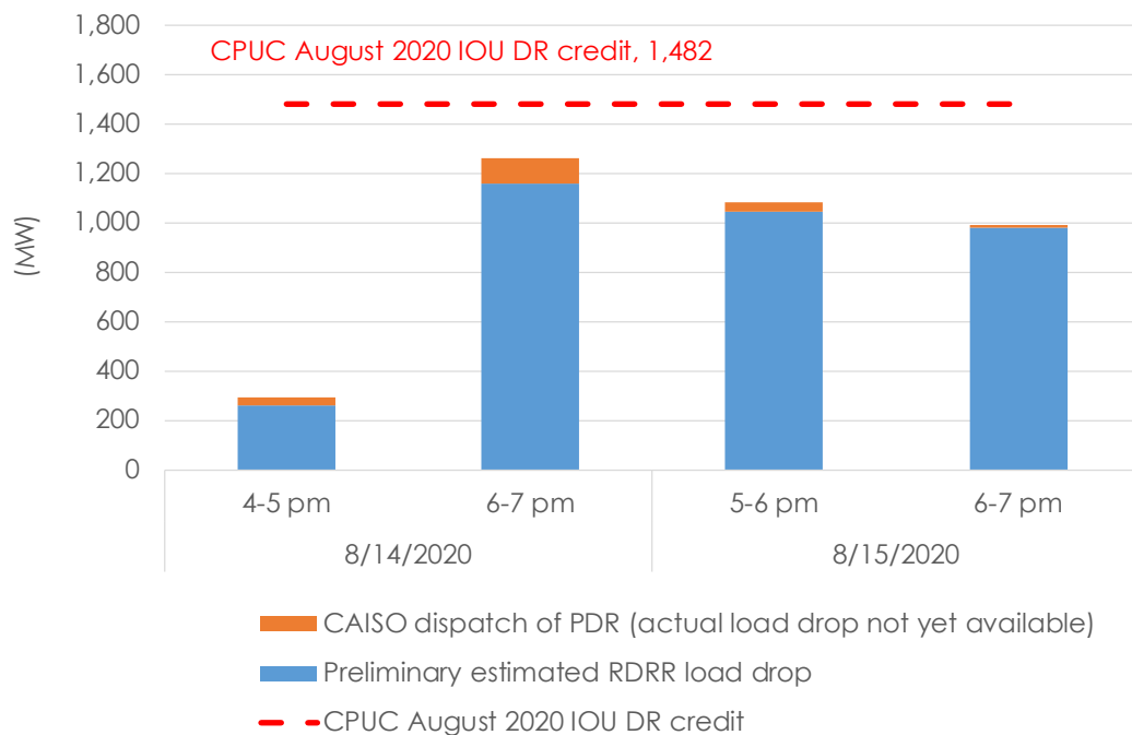
Figure 4.5: Credited IOU Demand Response: Preliminary Estimated RDERR Response and PDR Dispatch vs. CPUC August 2020 DR Credit
