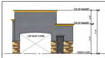
SOUTH ELEVATION
