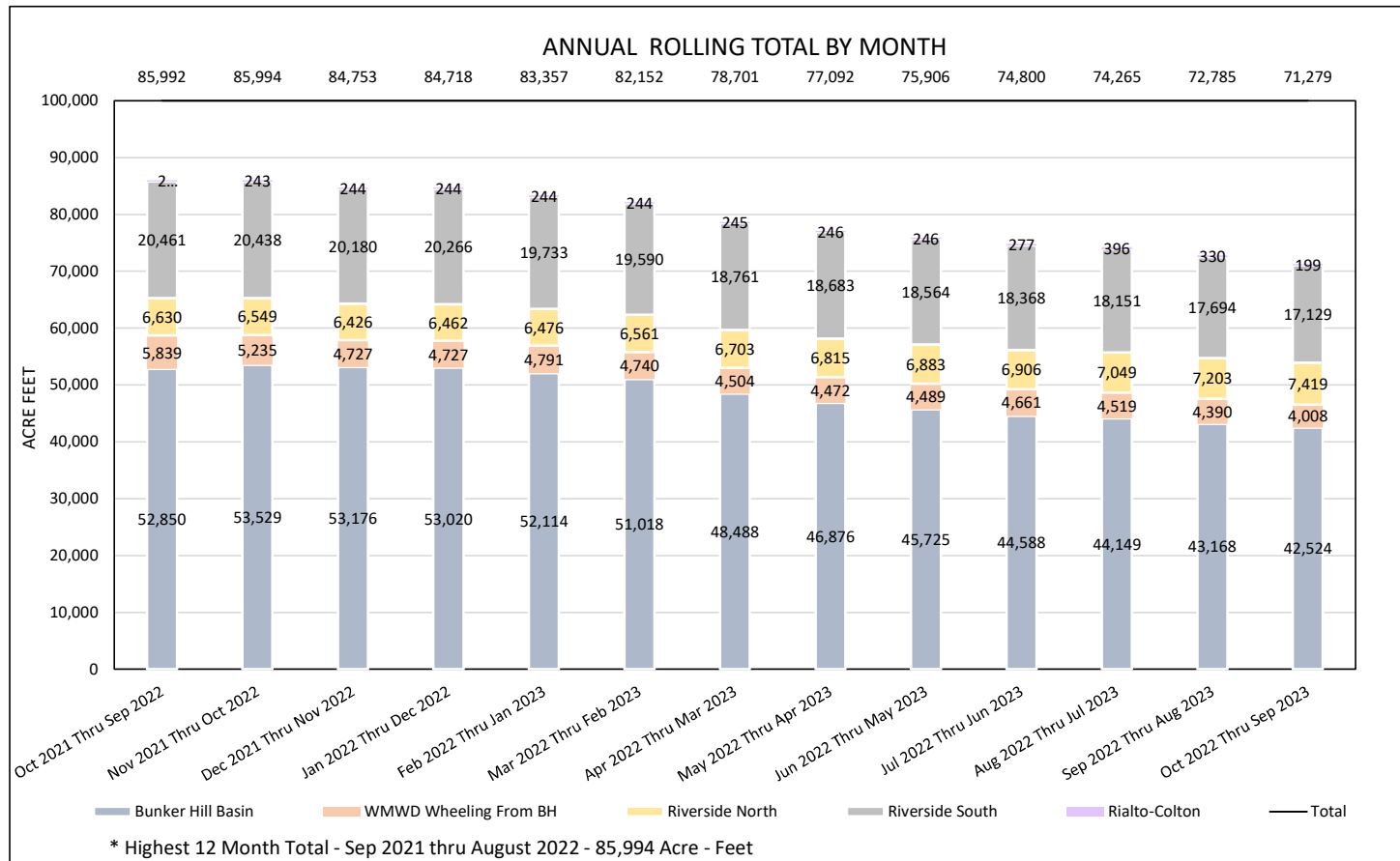
FIGURE 3: RPU WATER - TOTAL PRODUCTION REPORT
