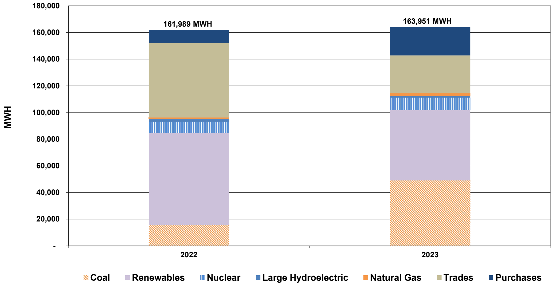
Chart 1 Total Energy Requirements/Resource Mix - January
