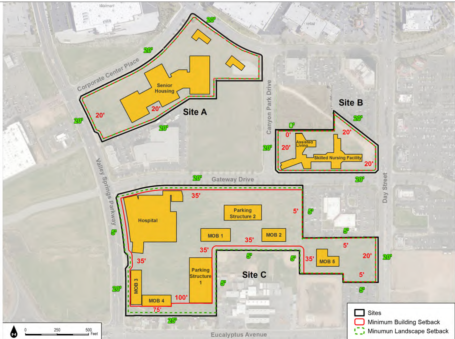
FIGURE 7-1 Site Setbacks
