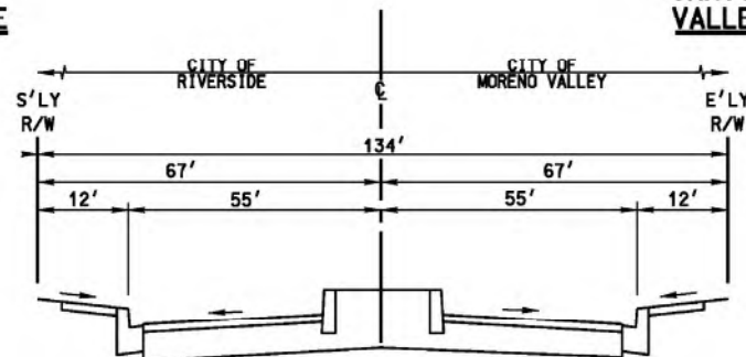
CLASS III BIKEWAY: THE BIKEWAY IS IDENTIFIED BY SIGNAGE ONLY DIVIDED MAJOR ARTERIAL ROAD PER THE CITY OF MORENO VALLEY
