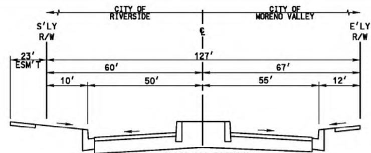
CLASS III BIKEWAY: THE BIKEWAY IS IDENTIFIED BY SIGNAGE ONLY DIVIDED MAJOR ARTERIAL ROAD PER THE CITY OF RIVERSIDE AND MORENO VALLEY DAY STREET N.T.S.
