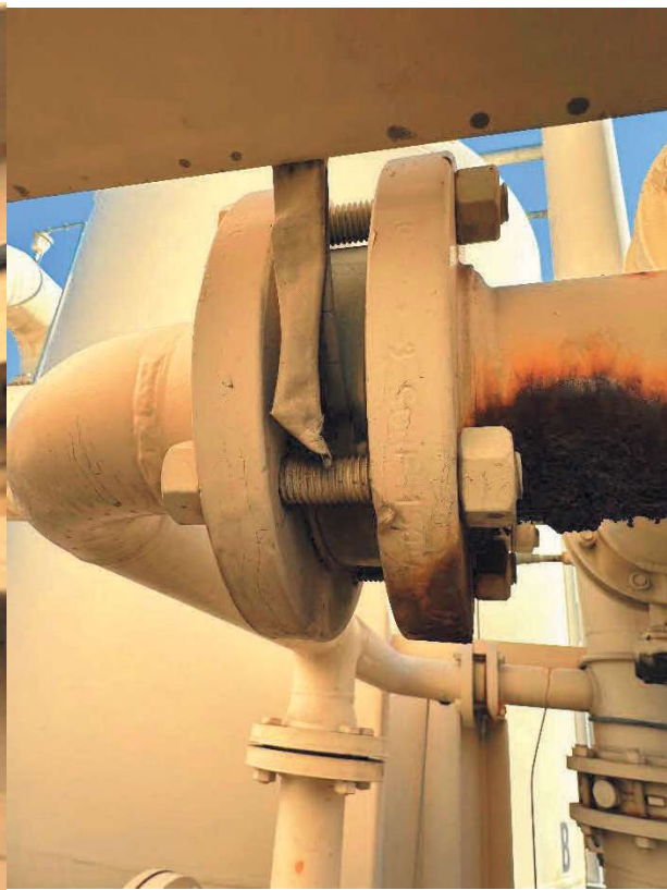
Vessel A – piping repair needs – reference pictures
