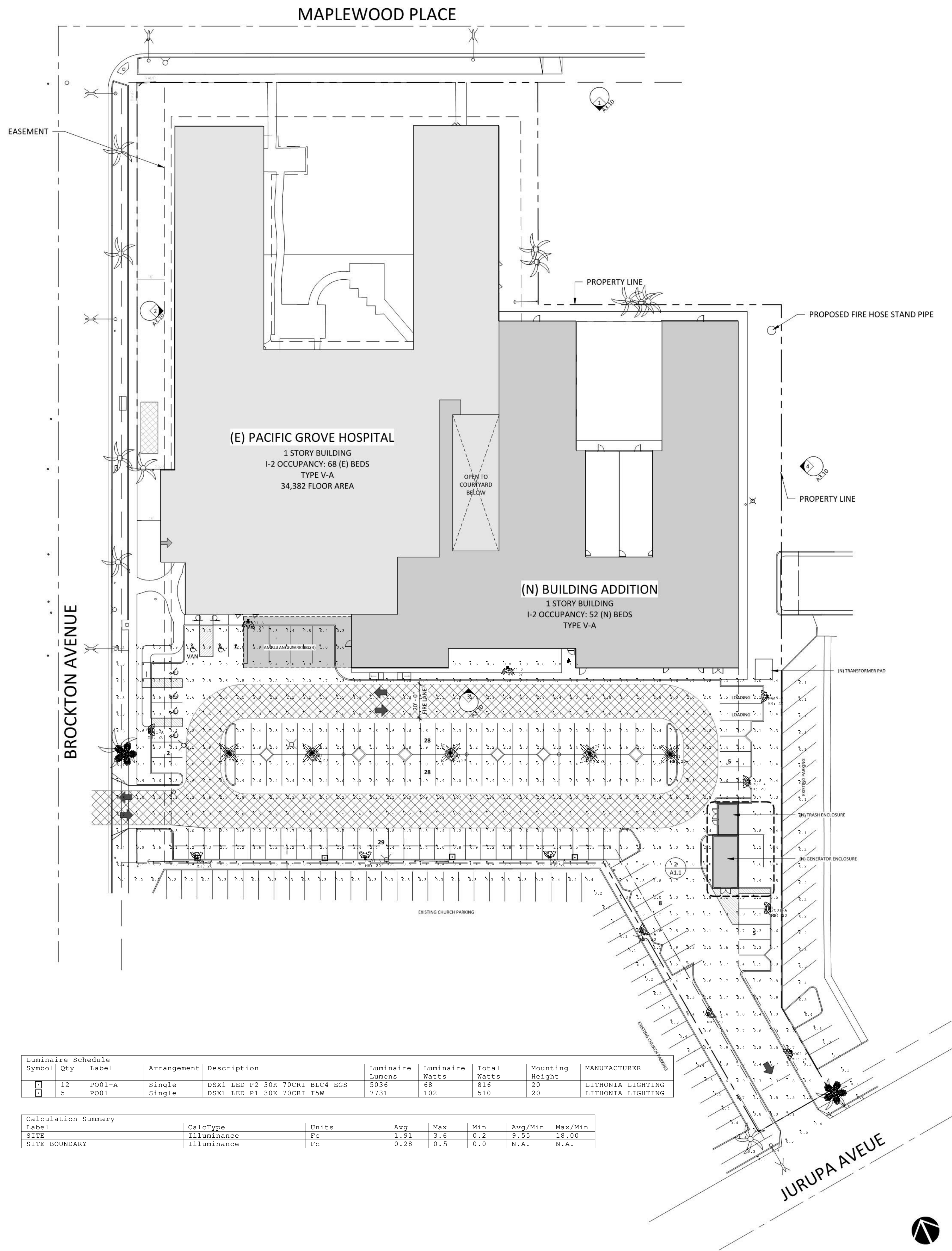
1 SITE PLAN - PROPOSED SITE A1.1 1" = 30'-0"
