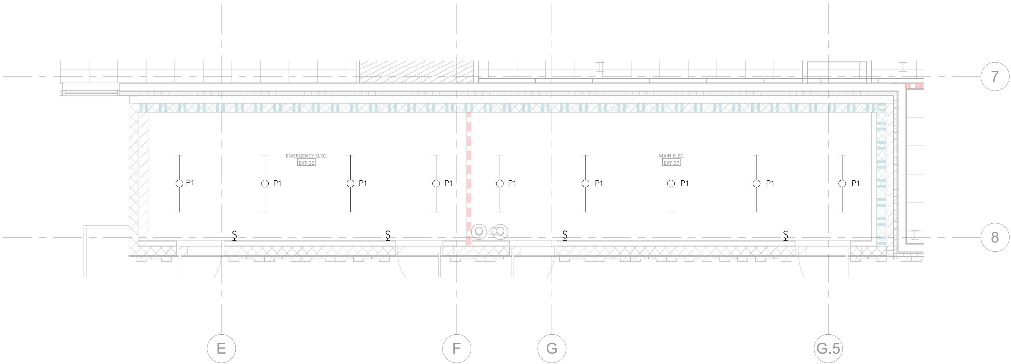
4 MAIN ELECTRICAL ROOM - LIGHTING PLAN SCALE: 1/4" = 1'-0"
