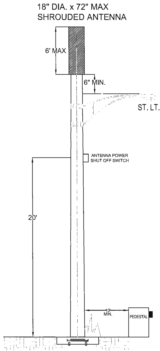
SPECIFICATION 2-6 UGS-800, 801, 802
