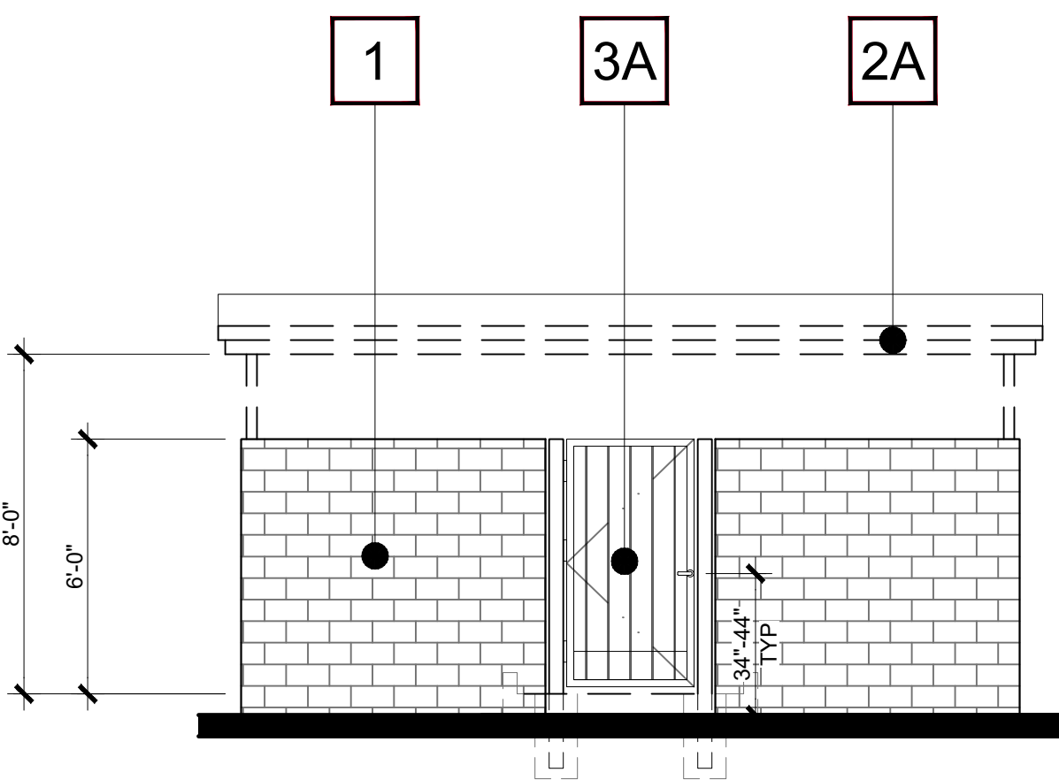
REAR ELEVATION 4
