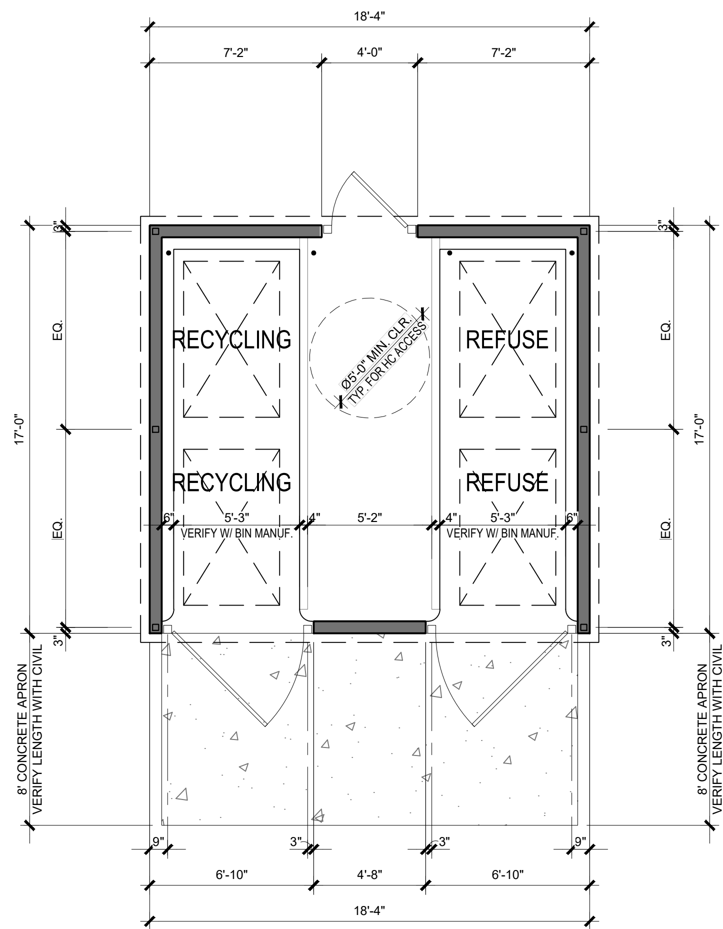
FLOOR PLAN 1
