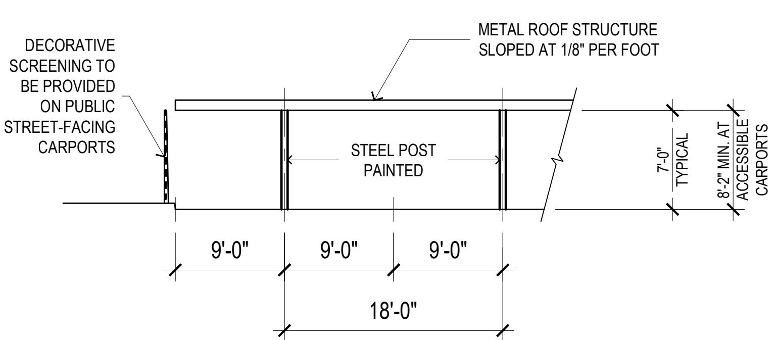
FRONT ELEVATION (TYP.) 1
