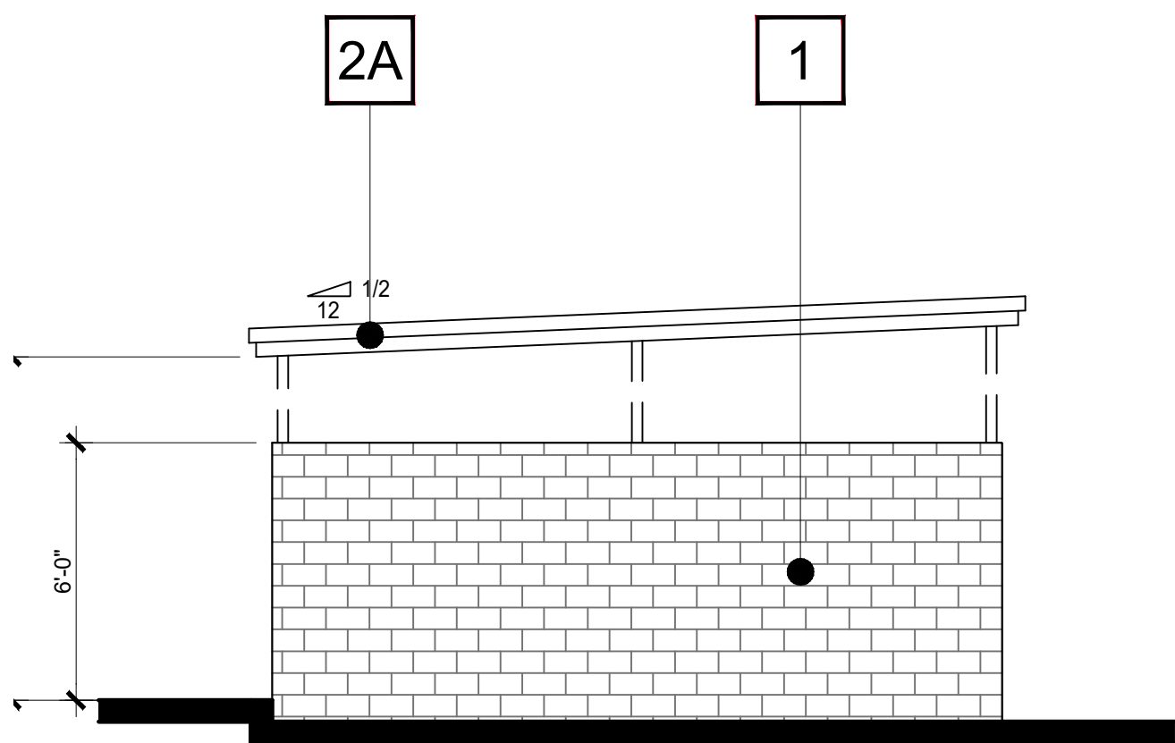
LEFT ELEVATION 3
