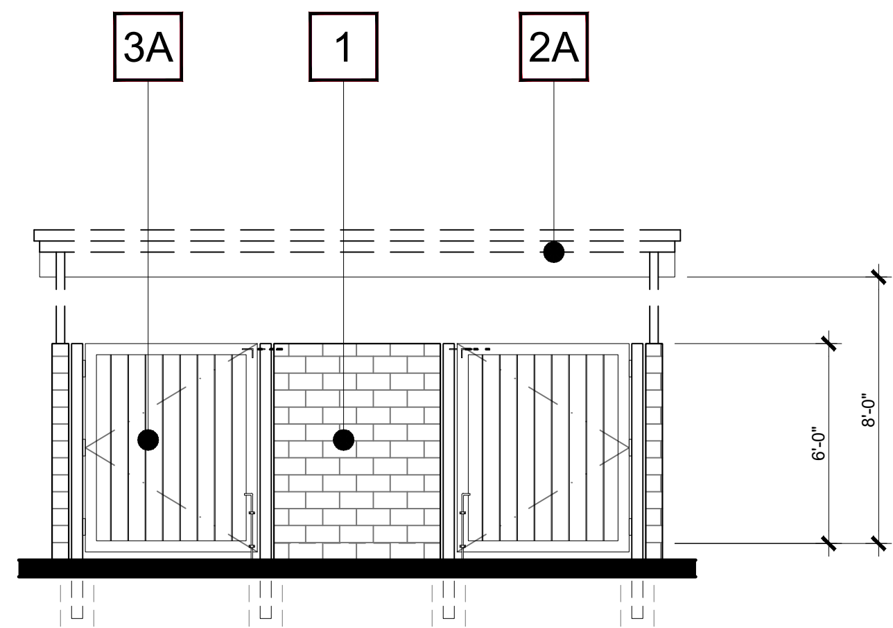
FRONT ELEVATION 2
