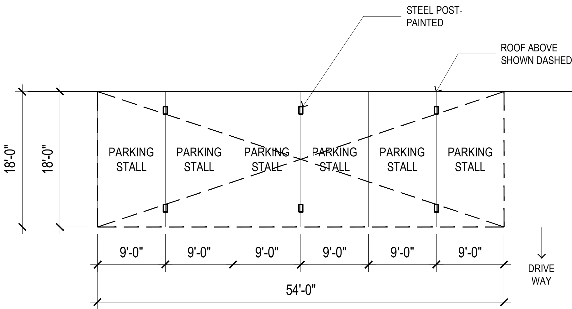
STANDARD CARPORT PLAN (TYP.) 3
