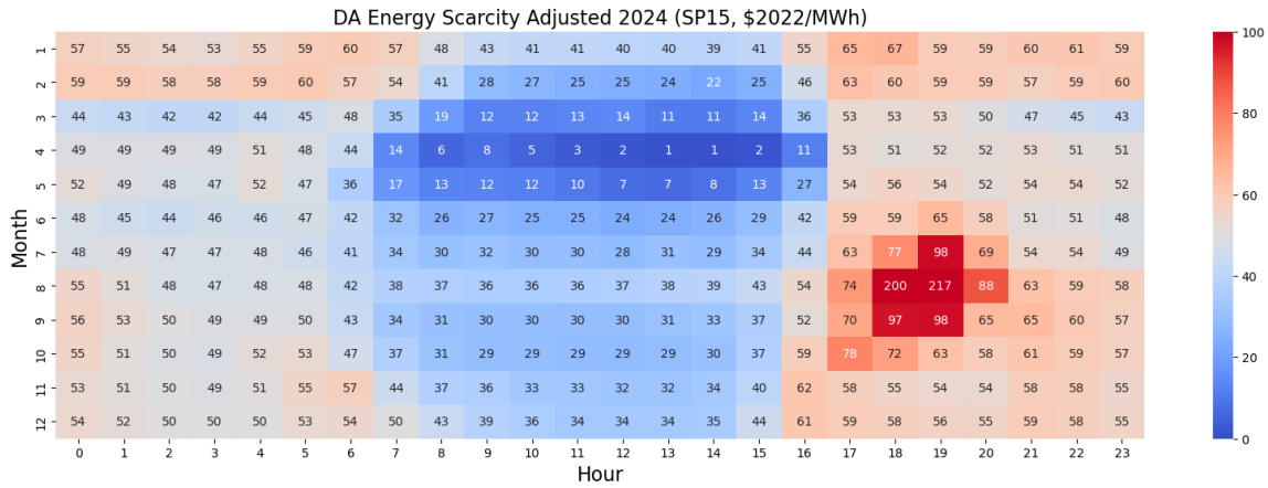
Figure 3-3. 2030 SP-15 Day Ahead Market Prices from SERVM
