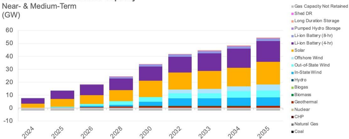
Figure 1-7. PSP capacity additions through 2035 7
