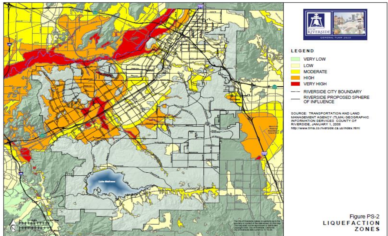
Figure 4.5.22 Liquefaction Zones
