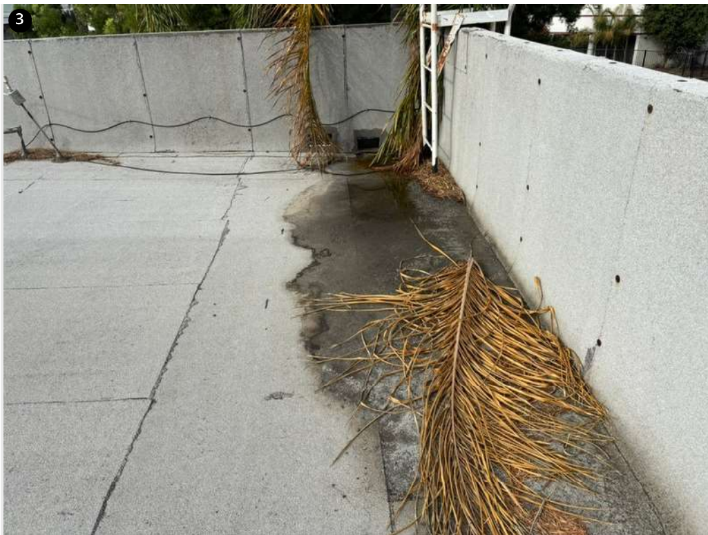
Ponding in northwest drain channel.
