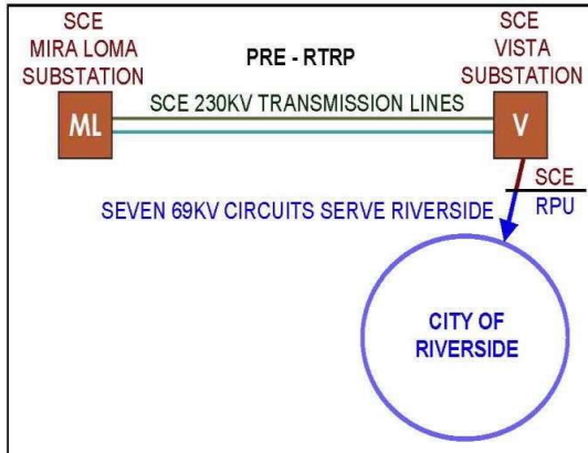
Single Connection to the State Grid
