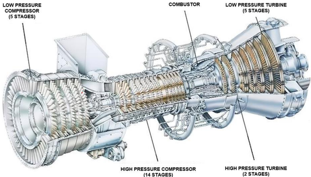
Image 1. GE LM6000
