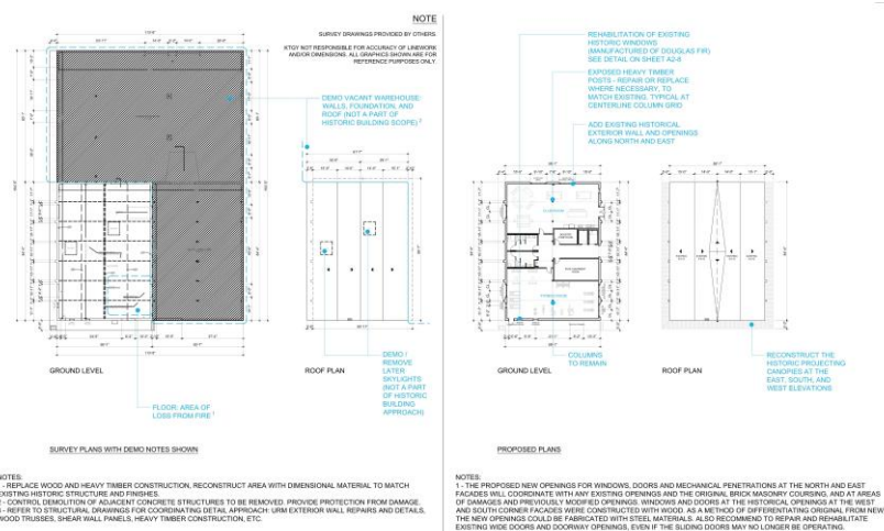
Barley Mills Building: Survey plans at left column and proposed plans at right column Source: ktgy/ Architecture + Planning Figure # D- 6
